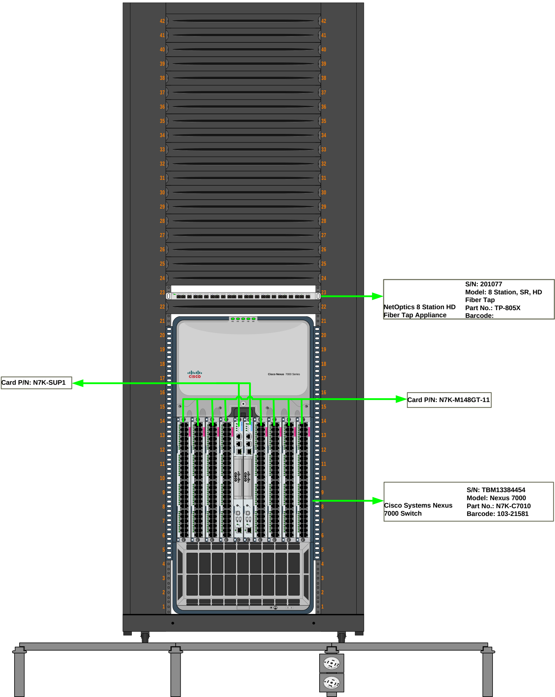
APC Rack 42 U, Model AR3350
